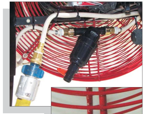
The filter mounts on the back of the fan (above), clears with a turn of the valve, and prevents water supply impurities from clogging nozzles (right).
