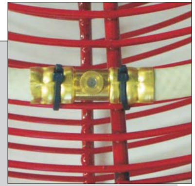
The filter mounts on the back of the fan (above), clears with a turn of the valve, and prevents water supply impurities from clogging nozzles (right).
